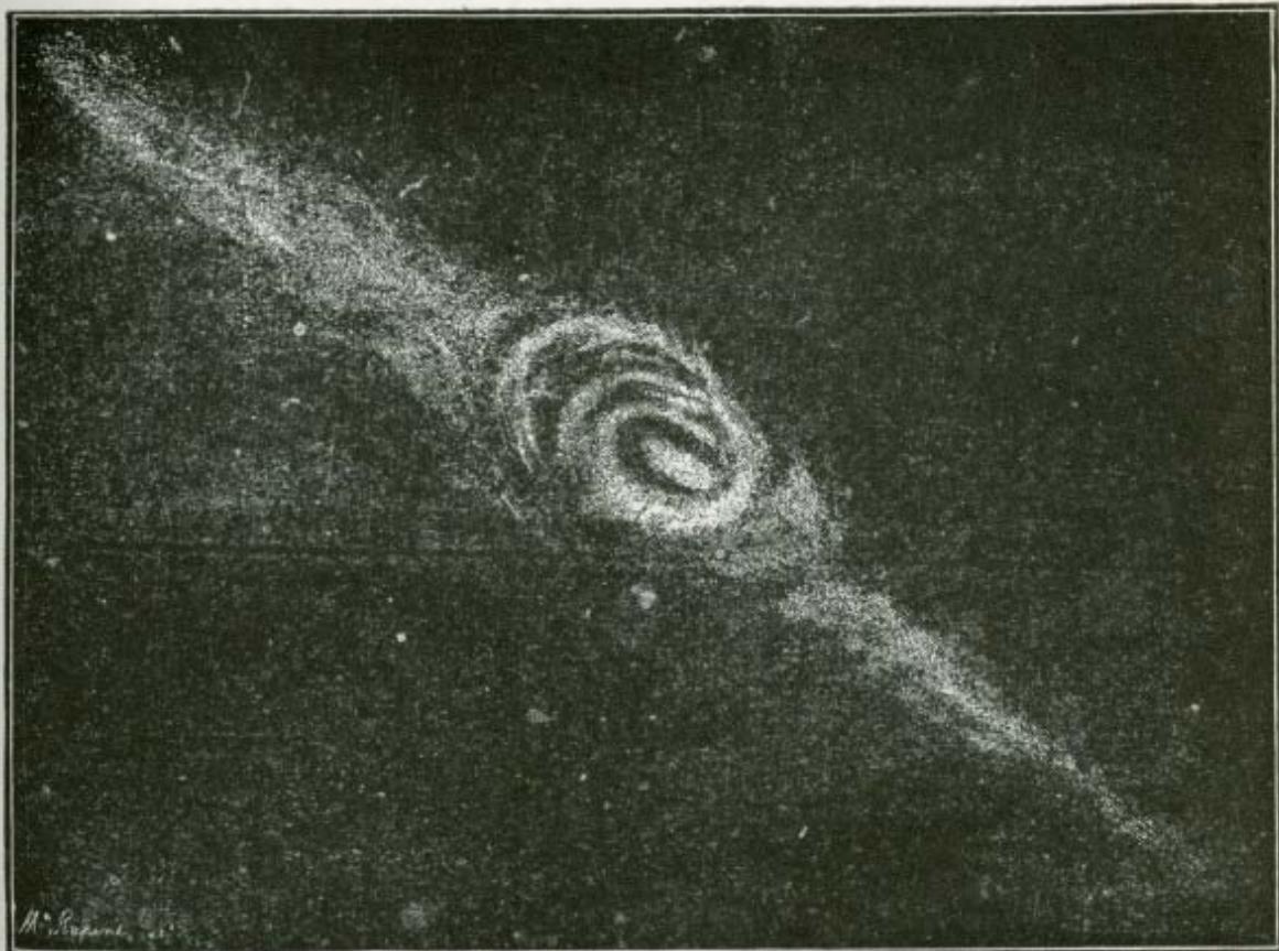
Nebula in the Lion.
